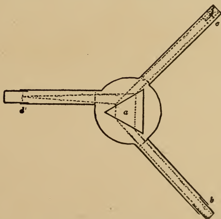
Fig. 75. PRINCIPLE OF THE SPECTROSCOPE.
